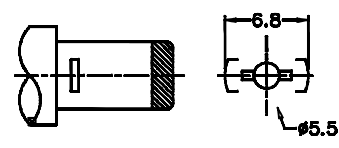
DC SPECIAL MATE PLUG
