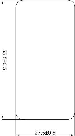
PANEL CUTOUT
