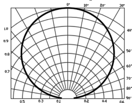
Radiation angle
