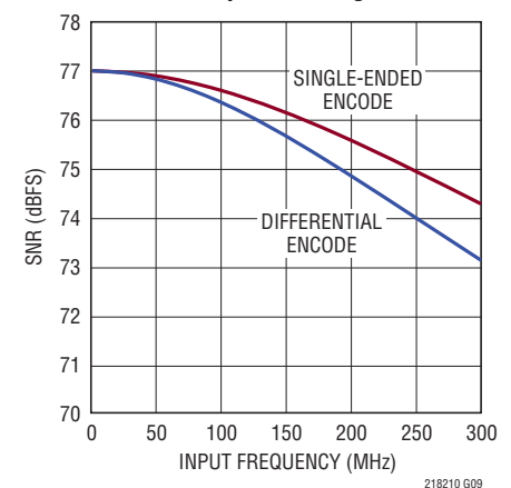
LTC2182: SNR vs Input Frequency, -1dB, 65Msps, 2V Range
