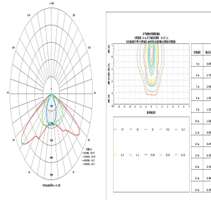
CURVE OF LIGHT DISTRIBUTION
