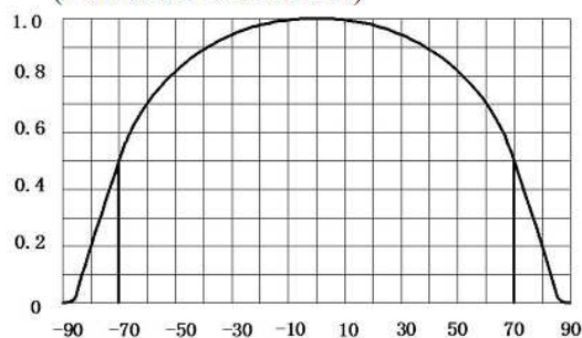
Fig.1- Light intensity distribution (Cartesian coordinates)
