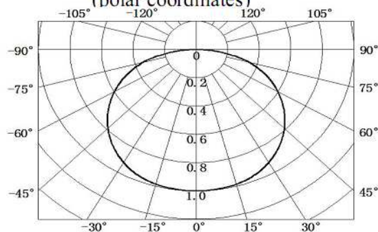
Fig.2- Light intensity distribution (polar coordinates)
