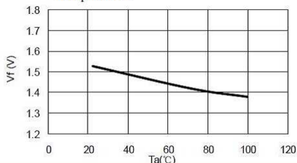
Fig.4-Forward Voltage(@350mA) vs. Temperature
