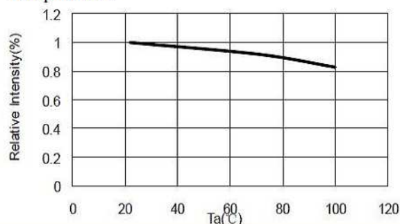
Fig.3-Relative Intensity (@350mA) vs. Ambient Temperature
