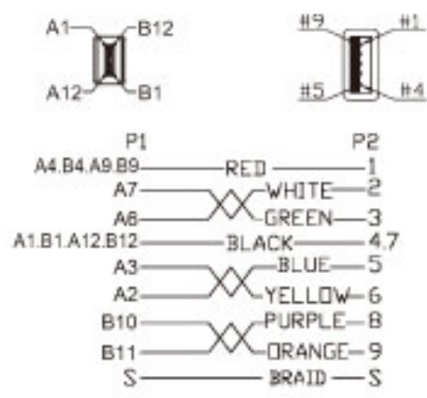
ZR070095 USB 3.1/C type plug to vUSB 3.1/A type plug cable (1M)
