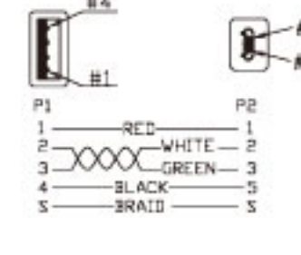
ZR070198 5P micro USB/B type plug & 8P Lightning plug to USB/A type plug cable (1M)
