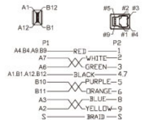
ZR070096 USB 3.1/C type plug to USB 3.1/B type plug cable (1M)
