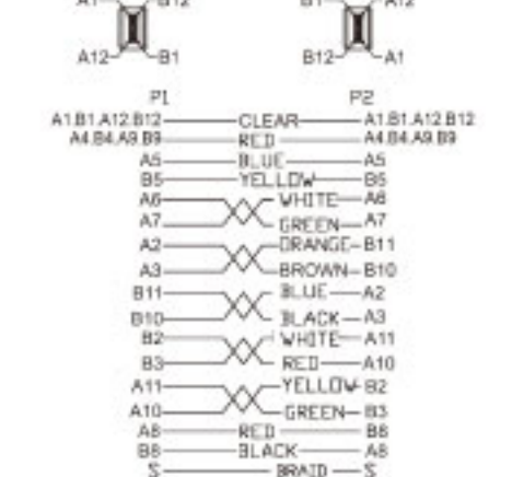
ZR070097 USB 3.1/C type plug to USB 3.1/C type plug cable (1M)
