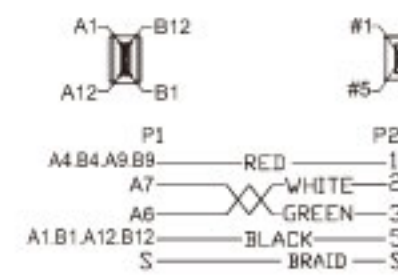
ZR070195 USB 3.1/C type plug to 5P micro USB 2.0/B type plug cable (1M)
