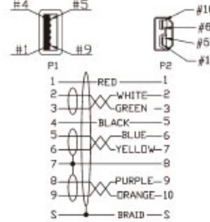
ZR070190 USB 3.0/A type plug to micro USB 3.0/B type plug cable (1M)
