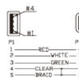
ZR070197 8P Lightning plug to USB/A type plug cable (1M)
