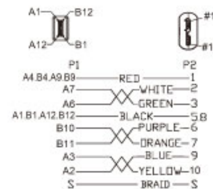
ZR070196 USB 3.1/C type plug to micro USB 3.1/B type plug cable (1M)
