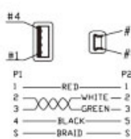
ZR07016 5P mini USB/B type plug to USB/A type plug cable (1M)
