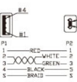
ZR07018 5P micro USB/B type plug to USB/A type plug cable (1M)
