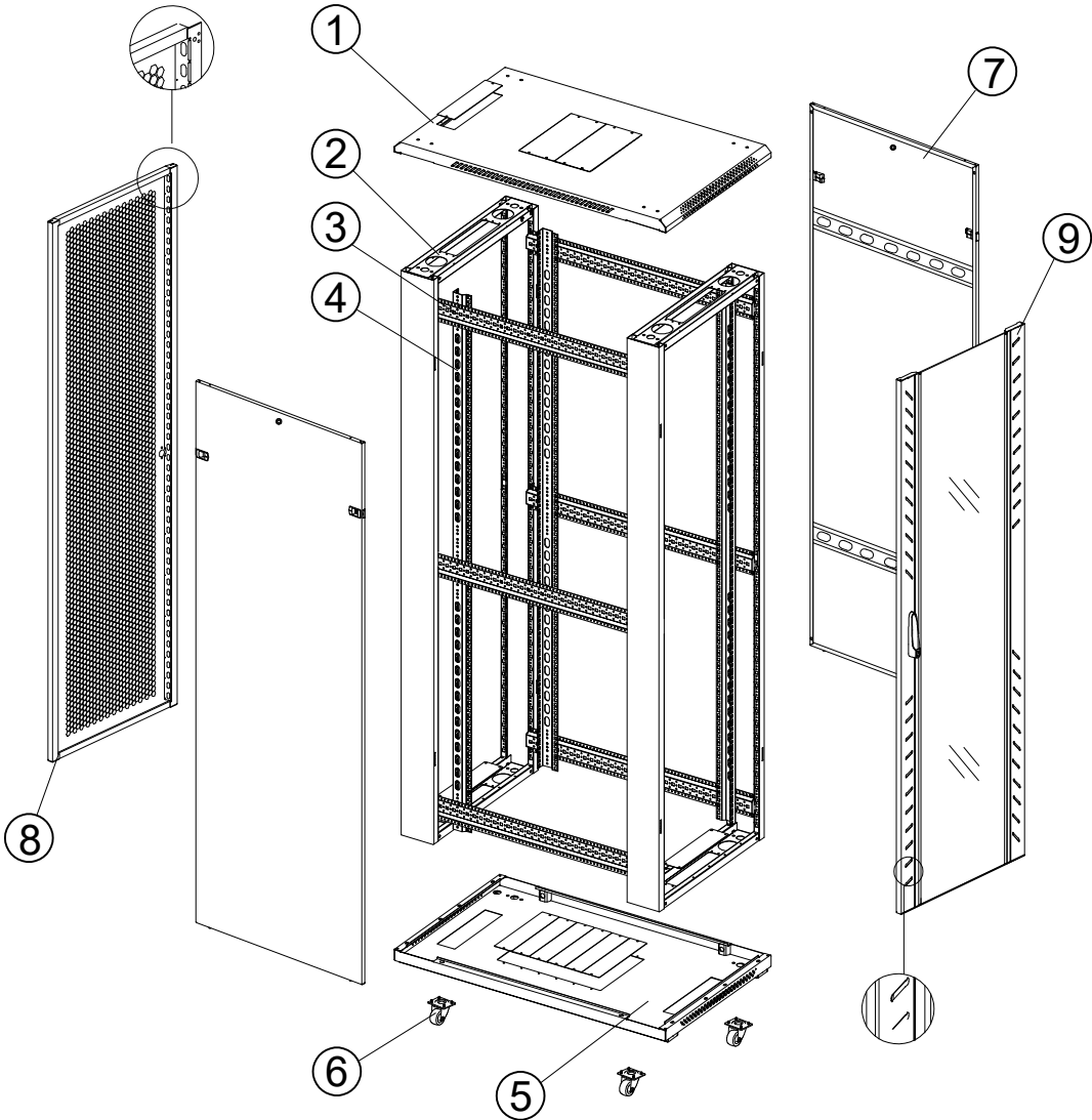
600mm Width Network Cabinet Exploded Drawing
