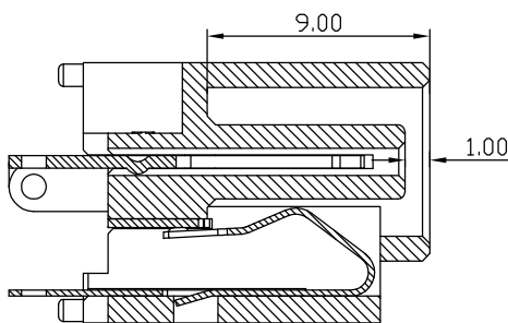
SECTION
