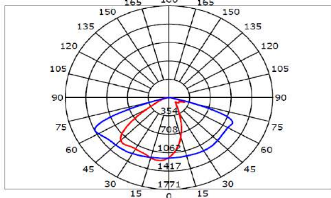
Luminous Intensity Distribution Curve
