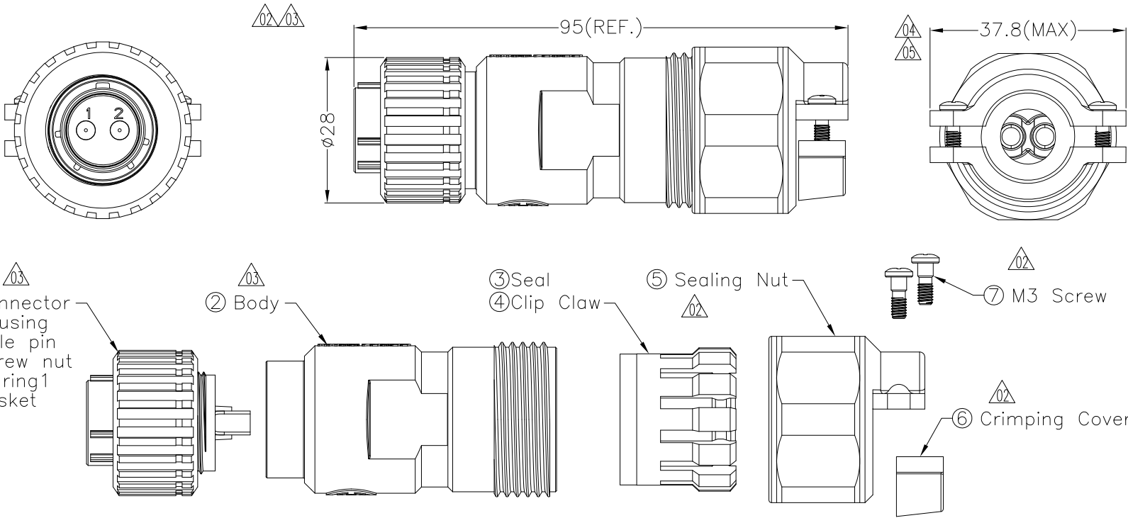
Explosion View
