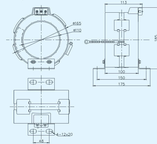
Fig 2. LXZK3-Φ 120
