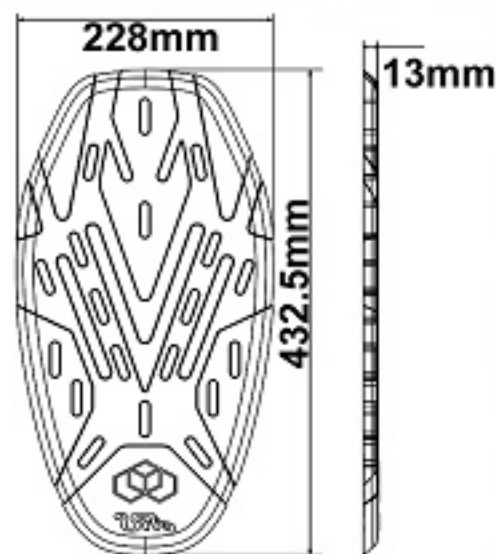
SR-B Back Protector
