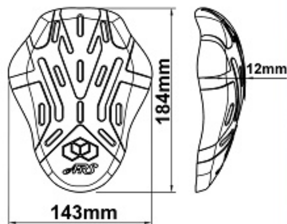
SR-S Shoulder Pads
