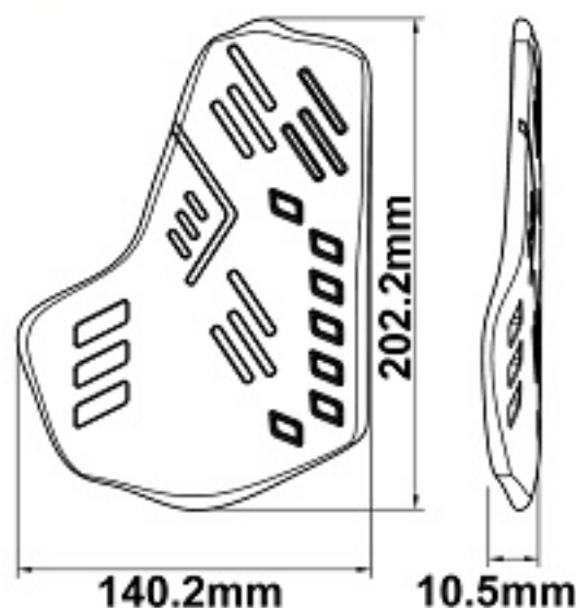
AP-CP1 Chest Protector
