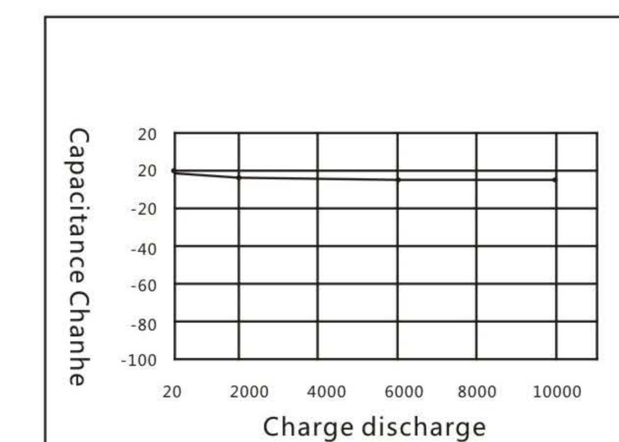
4. cycle life Characteristic-Cycle Time vs Cap Change
