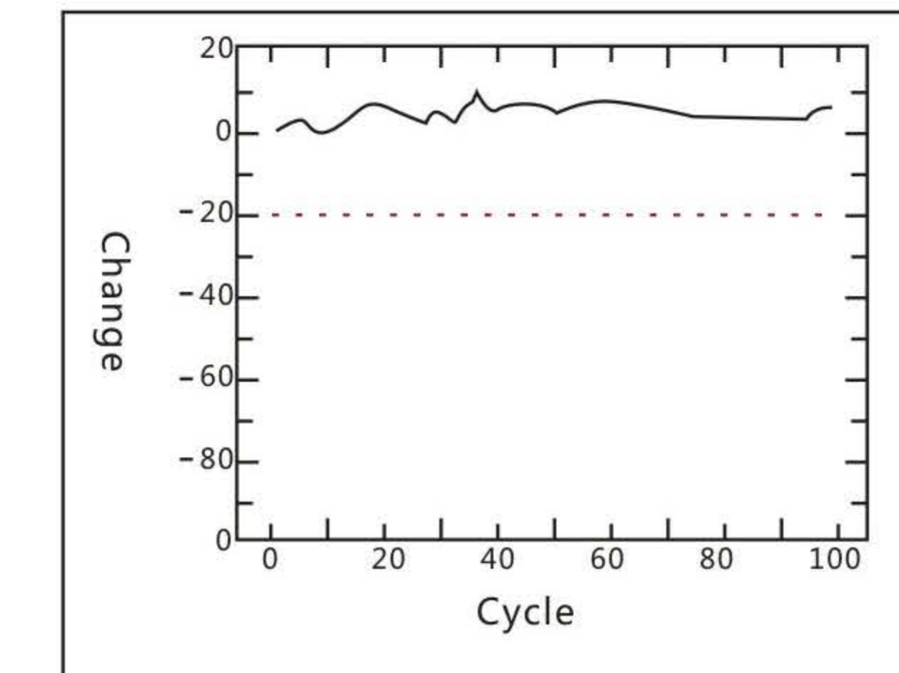
1. Cycle life Characteristic - Cycle Time vs Imp Change
