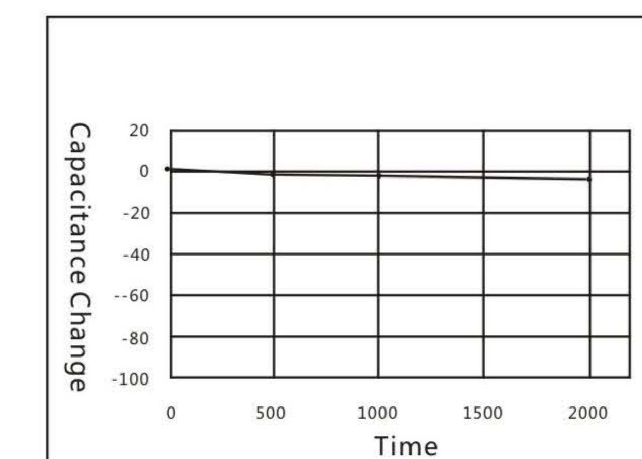
5. Load Life Test-Time vs Cap Change
