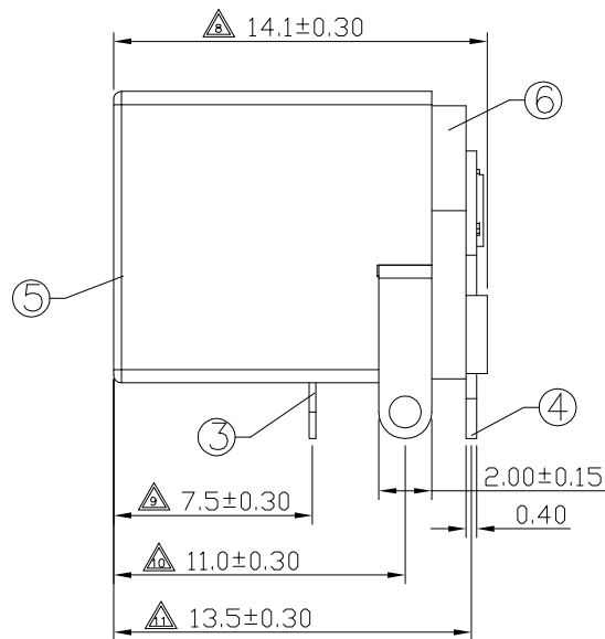
SCHEMATIC
