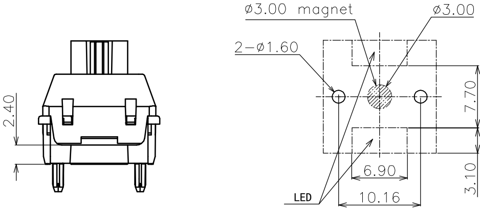
Recommended PCB Layout (Pattern Side)
