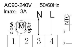
Water heating wiring diagram (do not connect terminal "close 4" of electric valve)
