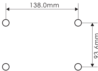
Installation Dimension
