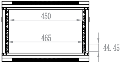
Mounting Dimension
