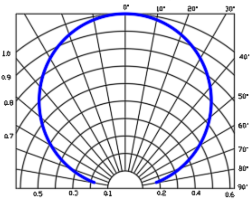
Radiation angle
