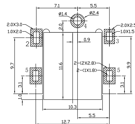
P.C.B LAYOUT TOP VIEW TOLRANCE:±0.05
