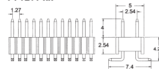
Pin header dual rows (SMD) YT127Pxx
