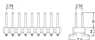
Pin header dual rows (SMD) YT254Pxx
