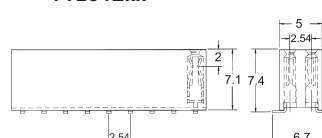
Female header dual rows (SMD) YT254Exx
