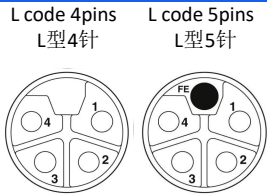
Pin assignment front view/孔位分布前视图
