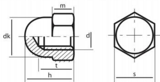
Hexagon domed cap nuts, high type
