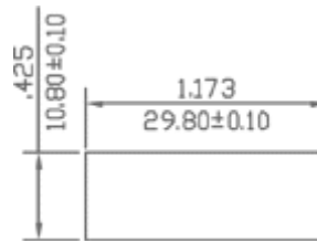
Mounting Hole of Snap-in Type
