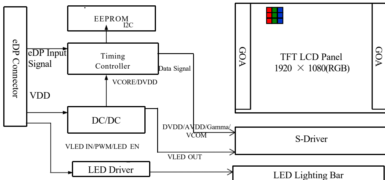
Figure 1. Drive Architecture
