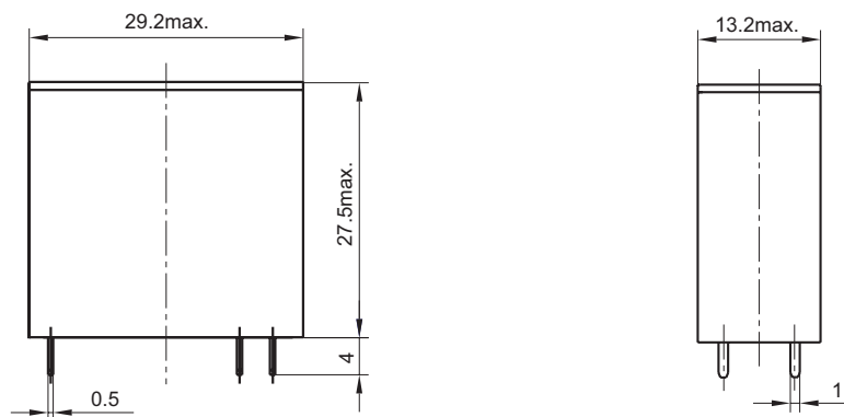
Outline Dimensions
