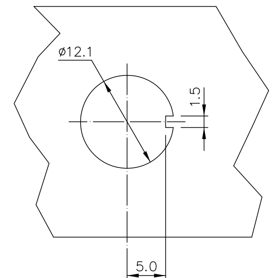
PANEL LAYOUT
