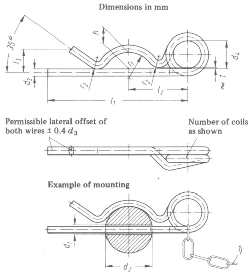
Description of a spring cotter for hole diameter d_1 = 5 mm as nominal diameter, galvanized. Spring cotter 5 DIN 11 024 — galvanized
