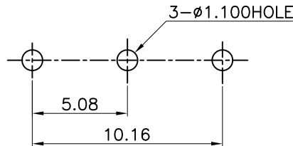
Recommended PCB Layout(Pattern Side) Top View tolerance: \pm 0.05\text{mm}
