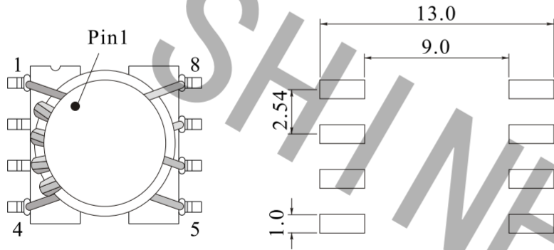
PCB Layout
