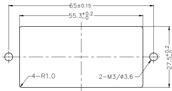
PANEL CUT-OUT
