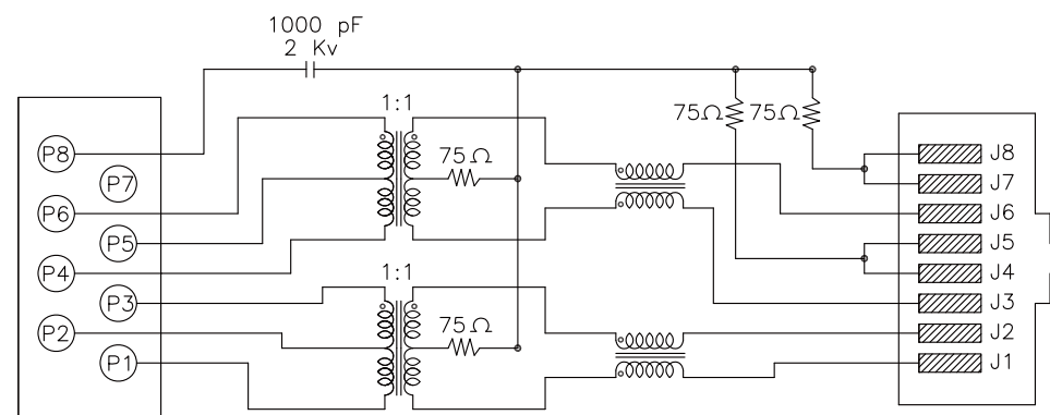
CONNECTOR SCHEMATIC
