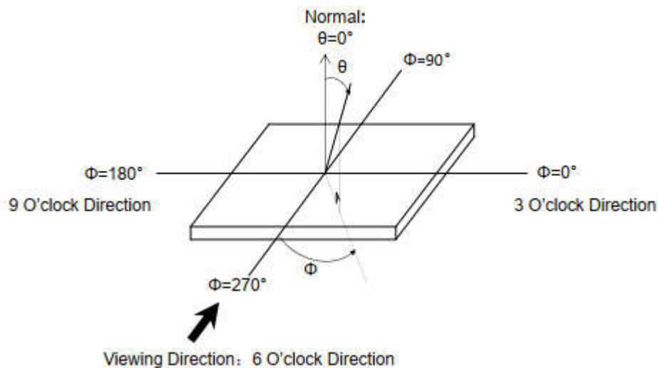
Definition of Viewing Angle \theta and \Phi
