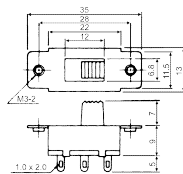
B1564 Slide switch (2P2T)
