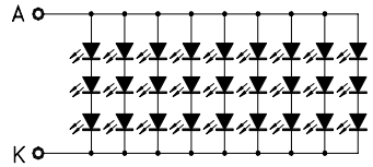
CIRCUIT DIAGRAM (LED 3x9=27 dies)
