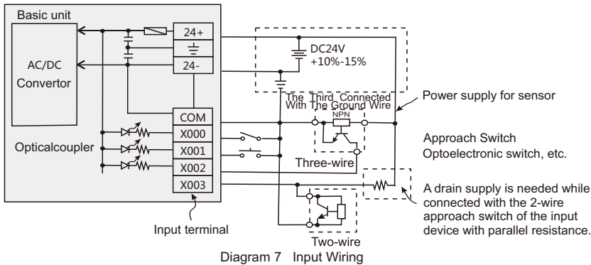
Diagram 7 Input Wiring
