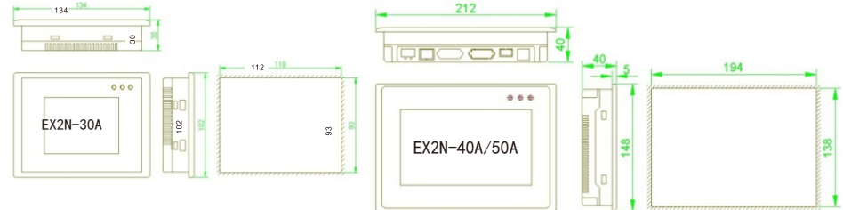
Diagram 1: Dimension Drawing
