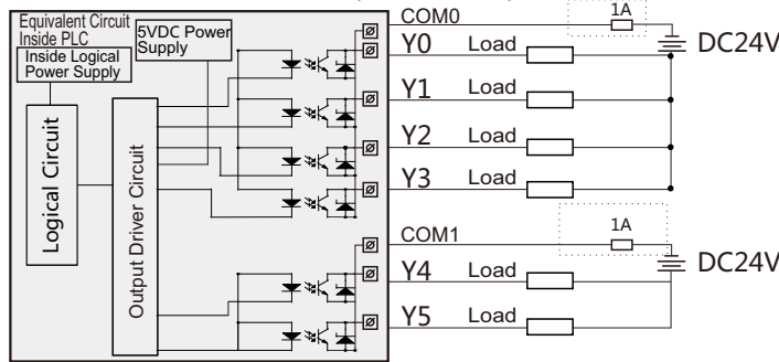
Diagram 9 Equivalent Circuit of Transistor Output
