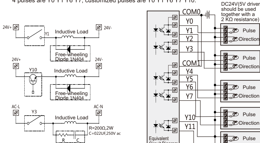
Diagram 10 Inductive Load Absorbing Circuit
