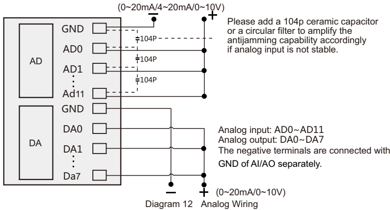
Diagram 12 Analog Wiring
