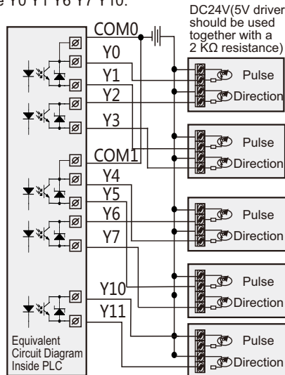
Diagram 11 Pulse wiring
