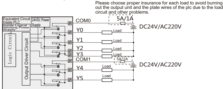
Diagram 8 Equivalent Circuit of Relay Output
