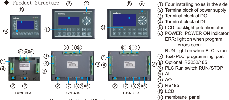
Diagram 2: Product Structure
