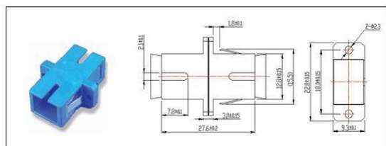
Figure1. SC Simplex Adapter
