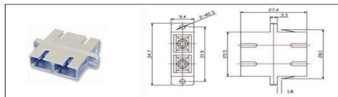
Figure4. SC Duplex Metal Adapter
