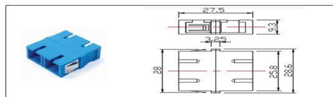
Figure5. SC Duplex Adapter without Flange
