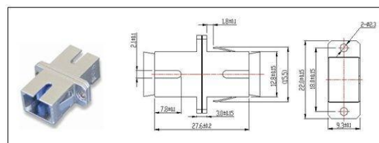
Figure2. SC Simplex Metal Adapter
