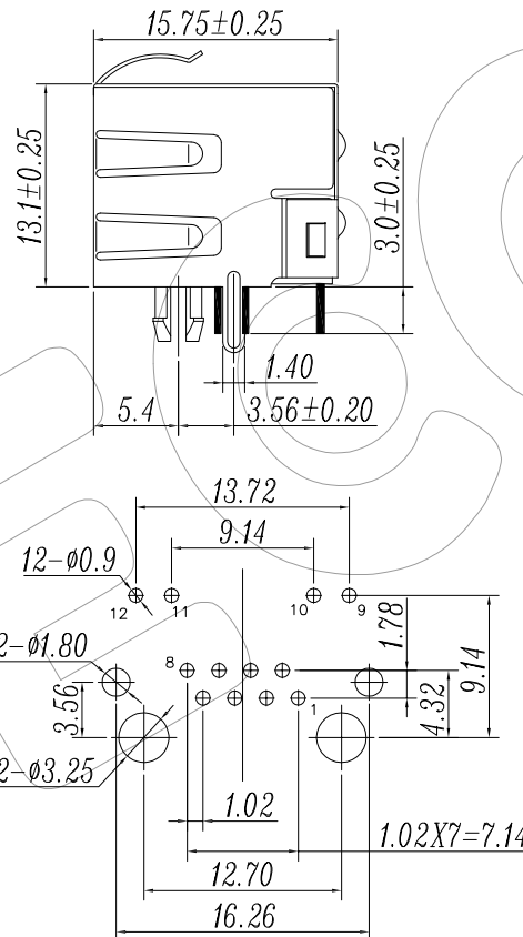
PC Board Layout Top View
