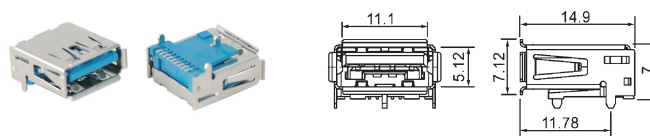
Y99001 USB 3.0/A type socket right angle
