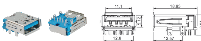
Y99004 USB 3.1/A type socket right angle
