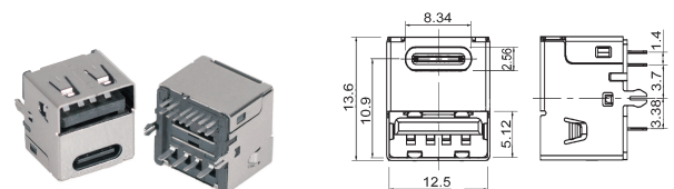
Y990075 USB/A type & USB 3.1/C type socket
