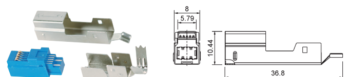
Y99016 USB 3.0/B type plug (molding type)
