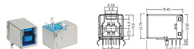
Y99012 USB 3.0/B type socket right angle
