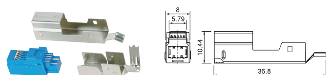
Y99016 USB 3.0/B type plug (molding type)
