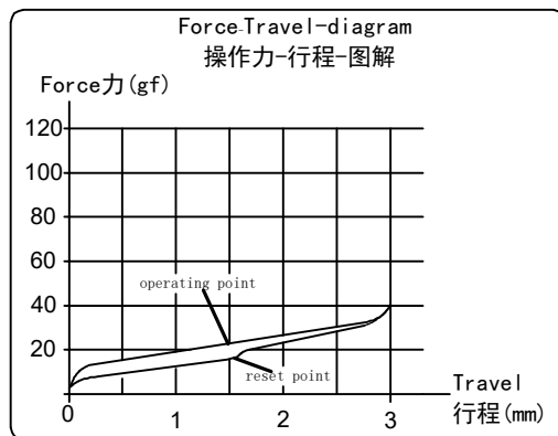
Linear actuation
