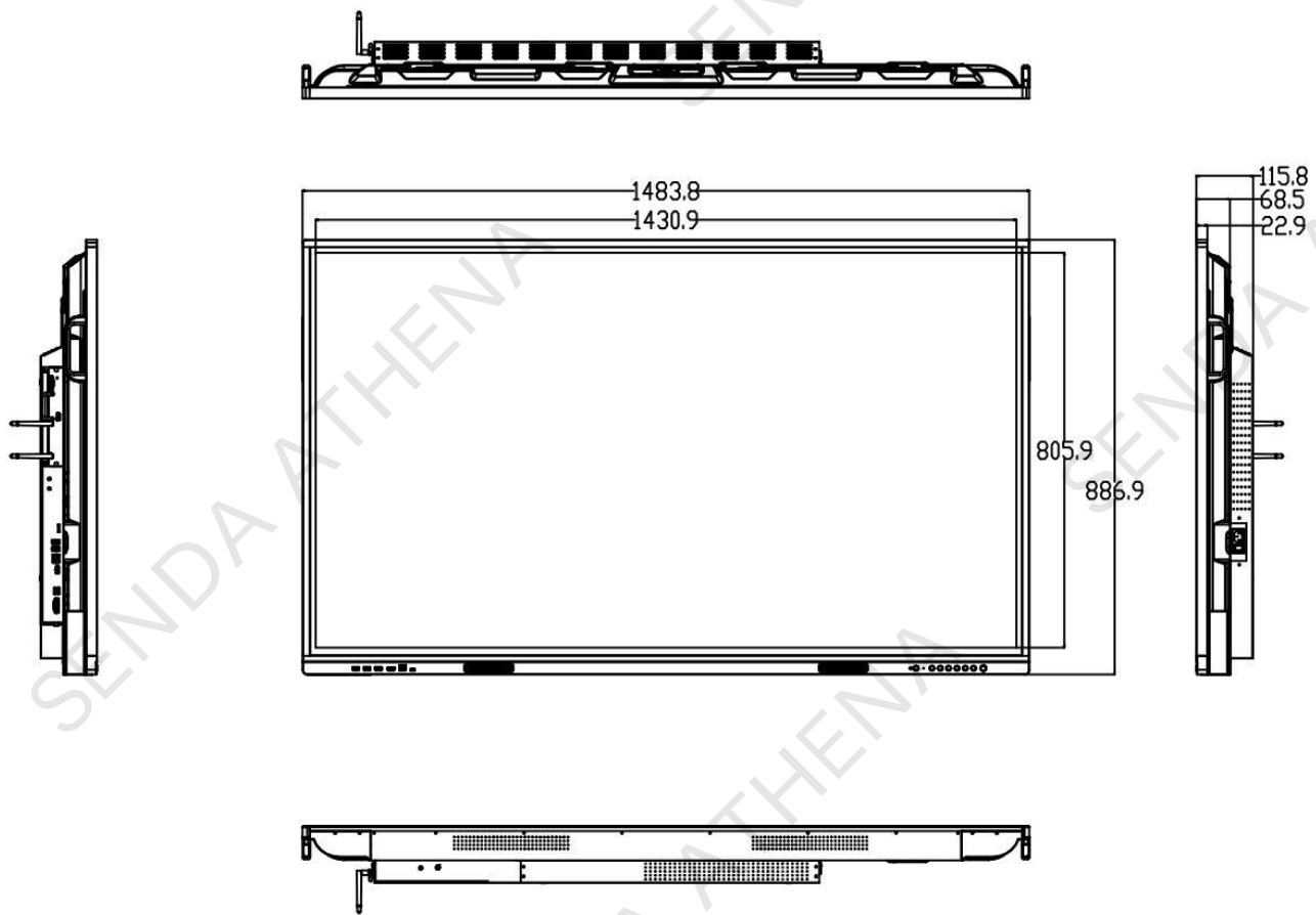
Front View
