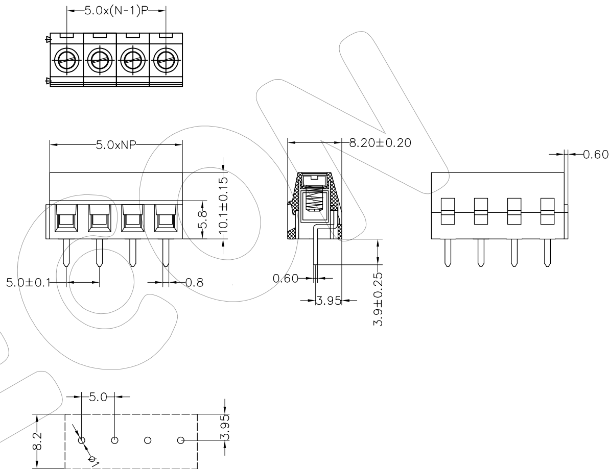
Recommended P.C.B Layout(Top Side)
