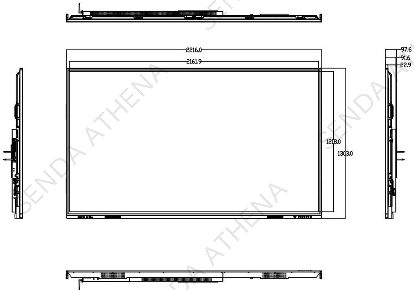
Front View
