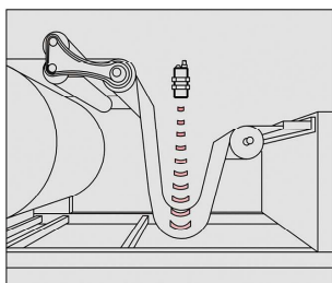
Control of sheet tension
