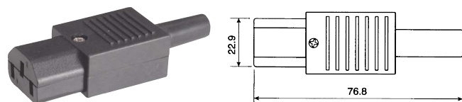
K24165U AC connector 250V 10A UL
