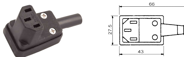
K24172U Right angle AC connector 250V 10A UL US
