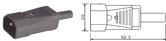
K24161U AC connector 250V 10A UL US
