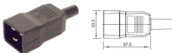
K24182 AC connector 250V 16A/20A UL US LISTED
