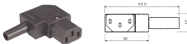
K24174 Right angle AC connector 250V 10A
