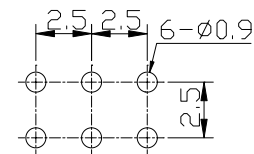
P. C. B LAYOUT
