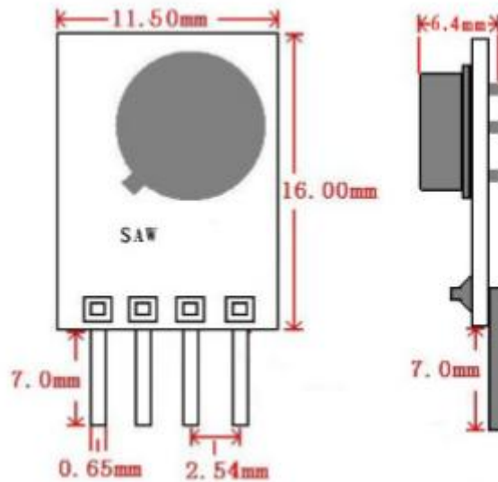
Figure2 CYT6 Dimension
