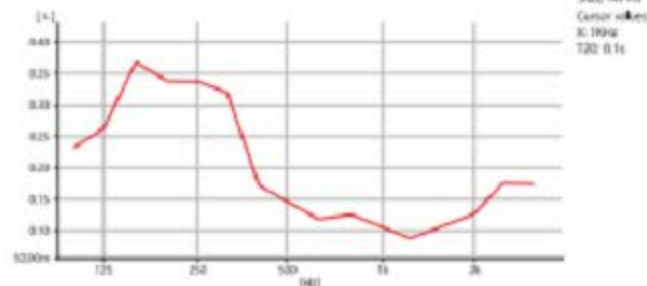
混響測試 Reverberation time test
