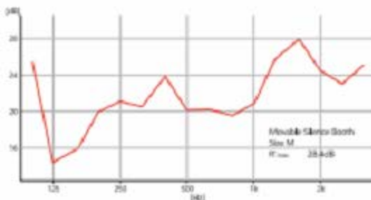
隔聲測試 Sound insulation test
